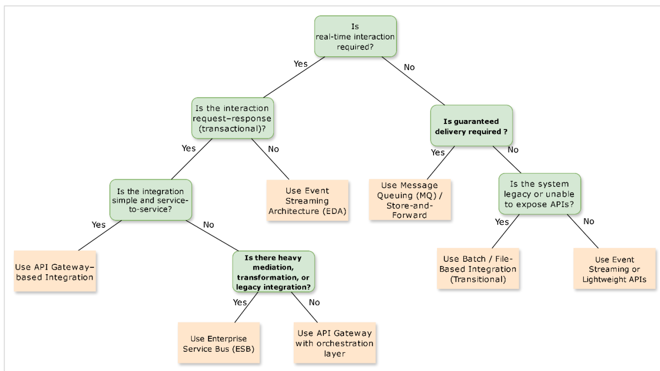
Figure 8 - Integration Pattern Decision Tree
