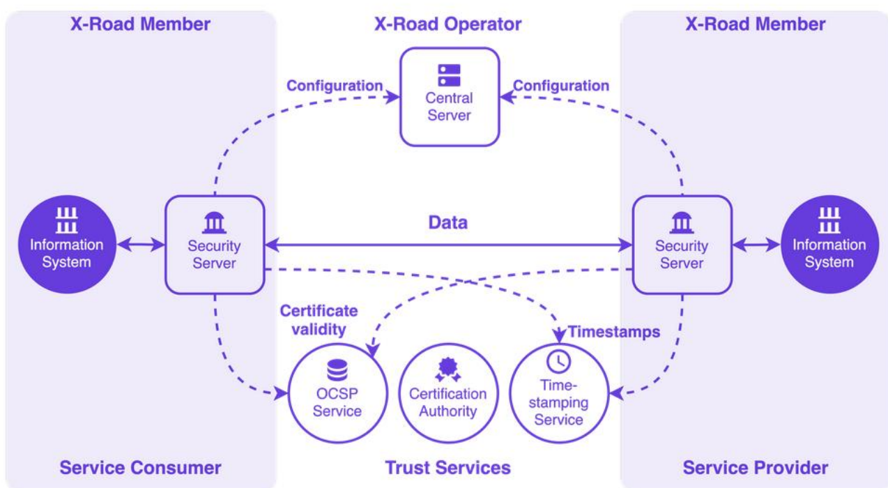
Figure 19 - X-Road Architecture
